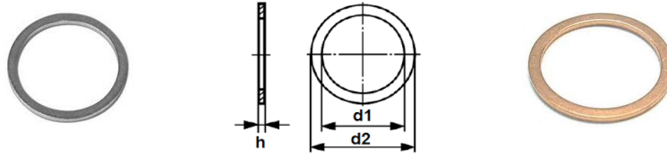
DIN 7603 A Aluminium Sealing Rings Available In The Following Sizes:
